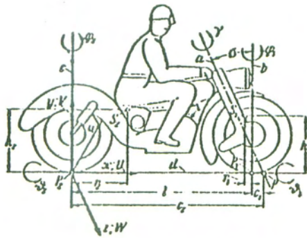
Fig. 1 Single-Track Vehicle
