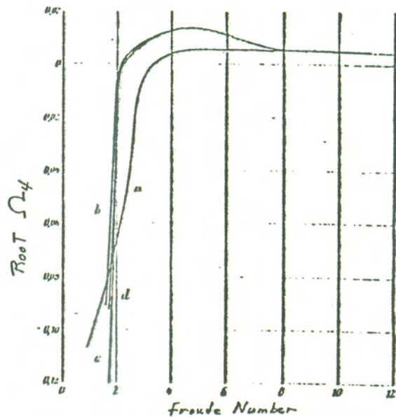
Fig. 15. Root \Omega_4 for the slow increase of deflection at high speeds as a function of Froude Number
