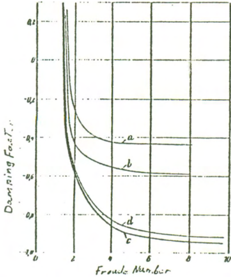
Fig. 12. Damping factor (real part of the roots \Omega_1 and \Omega_2 ) of the oscillation vs. Froude Number
