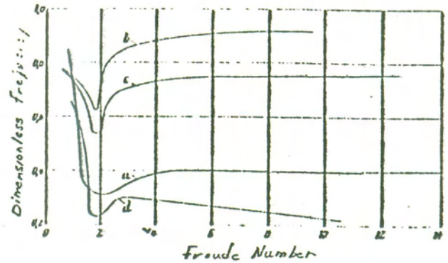
Fig. 13. Dimensionless frequency (imaginary part of the roots \Omega_1 and \Omega_2 ) of the oscillation as a function of Froude Number
