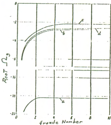
Fig. 14. Root \Omega_3 for return to null position as a function of Froude Number
