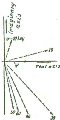
Fig. 8. Amplitude ratio \theta_2/\psi for the Vespa scooter for various speeds v . Dashed vectors for \theta_2/\psi with \psi = 1
