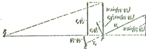
Fig. 3 Velocities for Single-Track Vehicle
