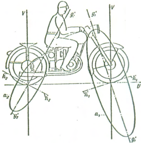
Fig. 5 Inertia ellipsoids of the Dürkopp MD 150 machine in the plane of the wheels Notation as in Fig. 4
