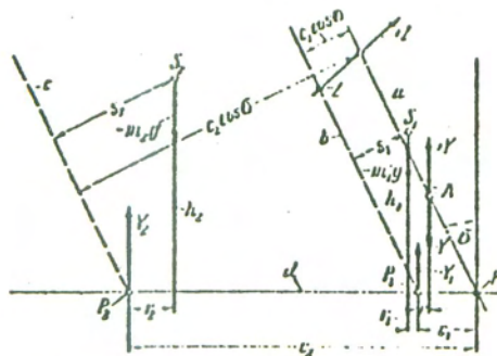
Fig. 2 Forces on Single-Track Vehicle
