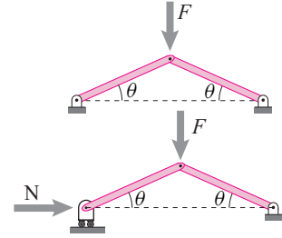
Figure 7.31: Two bars in a toggle mechanism.
