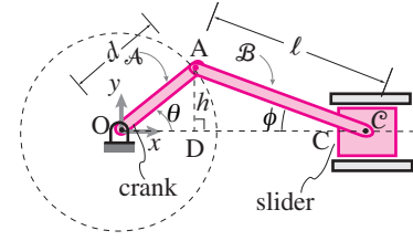
Figure 18.54: The slider crank mechanism.
