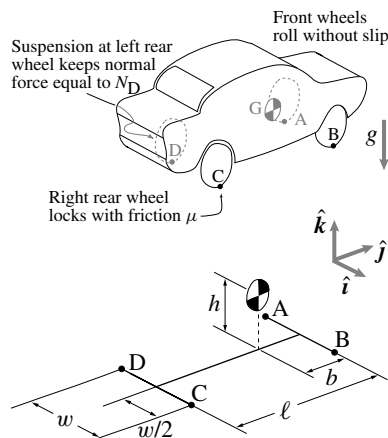
Problem 14.48: Given normal force at D, skidding at C.
