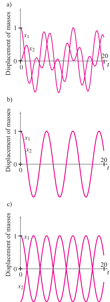
Figure 11.31: Motions of the masses from fig. 11.30 for three different initial conditions, all released from rest ( v_1 = v_2 = 0 ) a) x_1 = 1, x_2 = 0 , b) x_1 = 1, x_2 = 1 , and c) x_1 = 1, x_2 = -1 .
