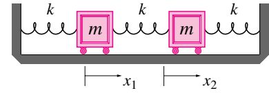
Figure 11.30: A two mass system. We define x_1 and x_2 so that the system is in equilibrium when x_1 = x_2 = 0 .
